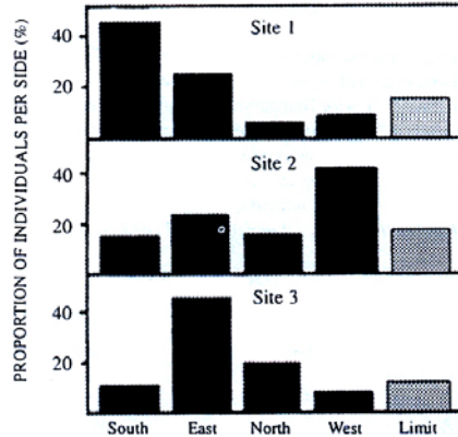
Fig. 6. Cardinal point orientation of Hamadryas spp. in the three sites (N=343).
