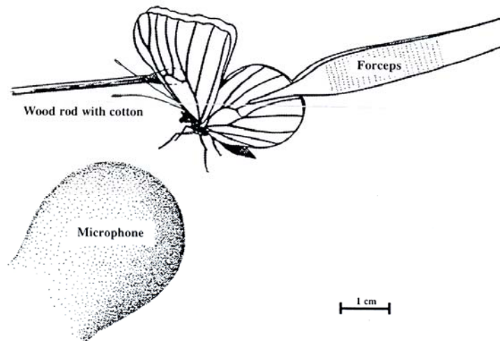
Fig. 9. Experimental procedure. A piece of cotton attached to a wood rod was intermittently introduced between the veins hypothesized to produce the sound. Sound intensity varied with cotton thickness, and normal clicks were produced when the cotton was removed.
