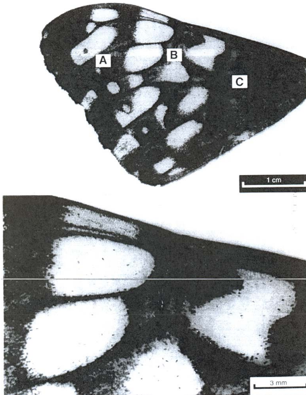
Fig. 1:2. The percussive pan of the sOllnd apparatlls is located in the mid frontal area of the forewing (B. detail below) Dampng effect decrea"cs as lhc cotton is moved lowards areas A and C.
