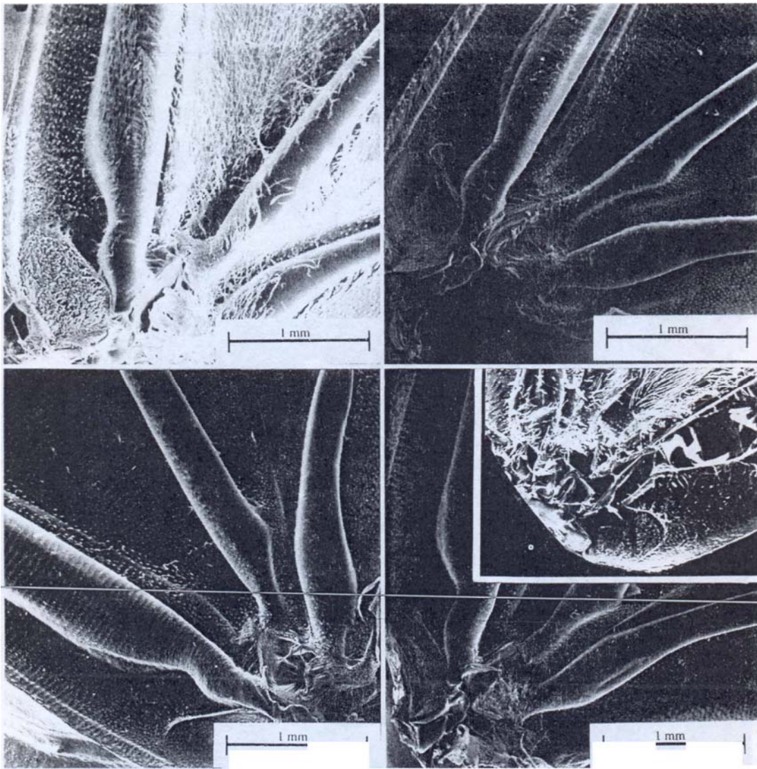
Fig. 16. Base of forewings of Hamadryas feronia (above: left female, right male) and Hamadryas februa (below: left female, right male, with enlargement of Venezuelan specimen by 10X).
