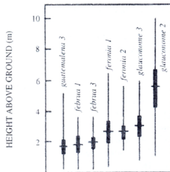
Fig. 4. Perching height of Hamadryas butterflies: range (vertical lines), standard deviation (bars) and mean (horizontal lines). Numbers: study sites (see text) (N=436)
