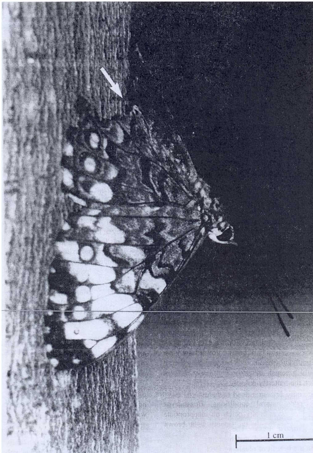
Fig.21 Severe wing damage (arrow) is not rare in wild Hamadryas males, but the sound-producing section often is in good condition.
