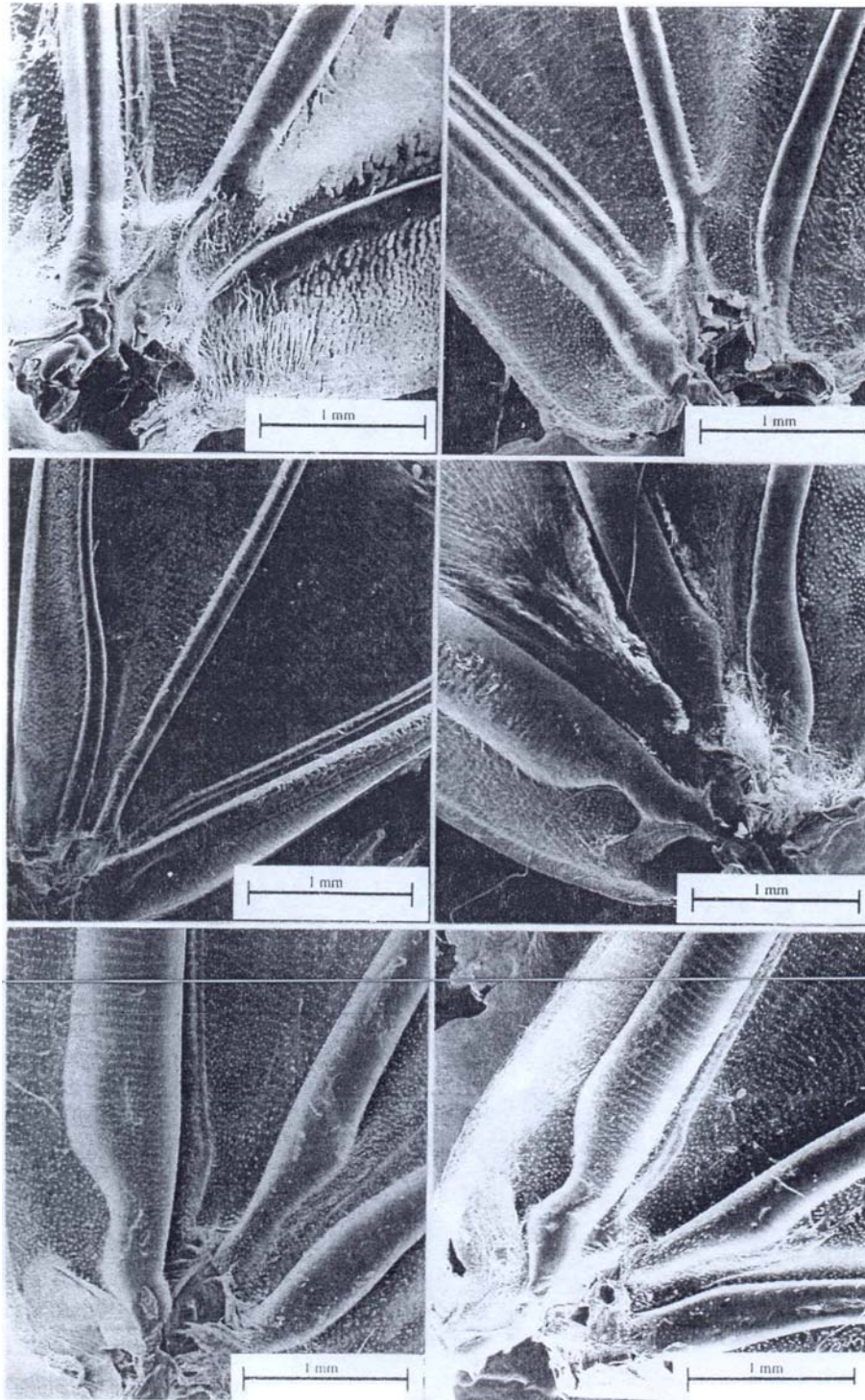
Fig. 15. Base of forewings of Siproiea stelenes (above, left female, right male), male Ectima thecla (middle left), male Hamadryas glauconome (middle right) and Hamadryas guatemalena (below: left female, right male)
