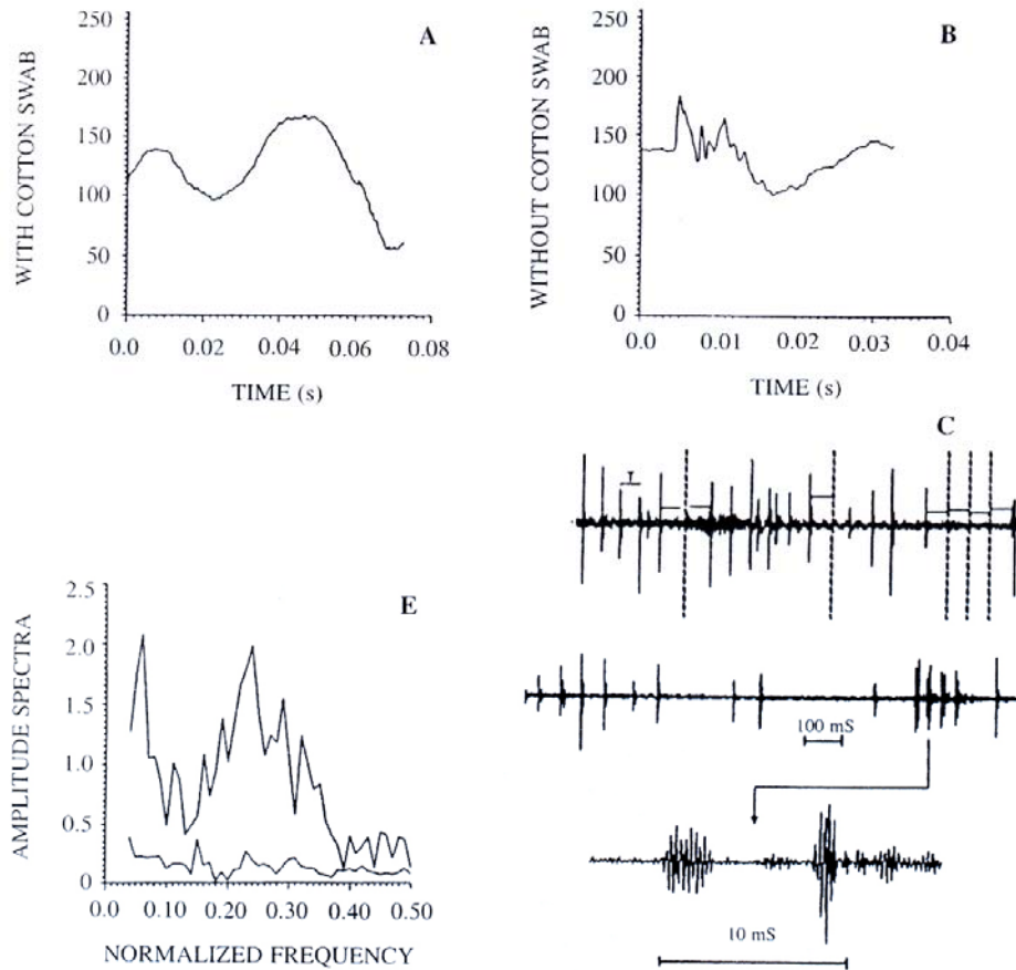
Fig. 11. A, B. The experimental intrusion of cotton between the percussive veins decreases the intensity of the clicking sounds. This is audible to the human ear and also shows in the sonogram. C. When some expected clicks are missing in a sequence, the distance between produced clicks preserves the expected intervals (T). Apparently the insect controls the emission of sound by changing wing movement: to click, the wings are clapped. D. When 2-3 individuals interacted, the intervals diminished, suggesting that several individuals were simultaneously emitting sound (detail enlarged). E. The peak amplitude of the click occurs at frequencies of 1.3-3.8 kHz. Amplitude in arbitrary units for all figures. For the amplitude spectra: above: signal, below: noise.
