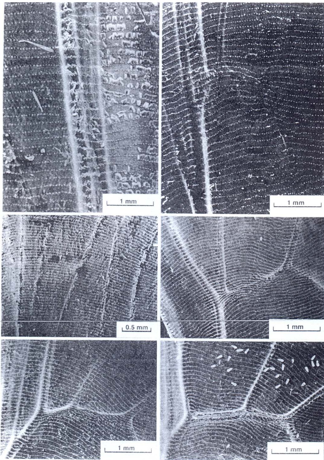
Fig 13. Forewing veins in Siproeta stelenes (above, lefts male, right female) male Ectima thecla (middle left), male Hamadryas glauconome (middle right) and Hamadryas guatemalena (below: left female, right male)
