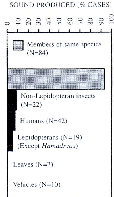
Fig. 20. Production of sound by Hamadryas spp. in response to a variety of stimuli, including falling leaves and human observers. Some perches were on roadside trees, so the reaction to vehicles passing in front of perches was also recorded. (N=184).
