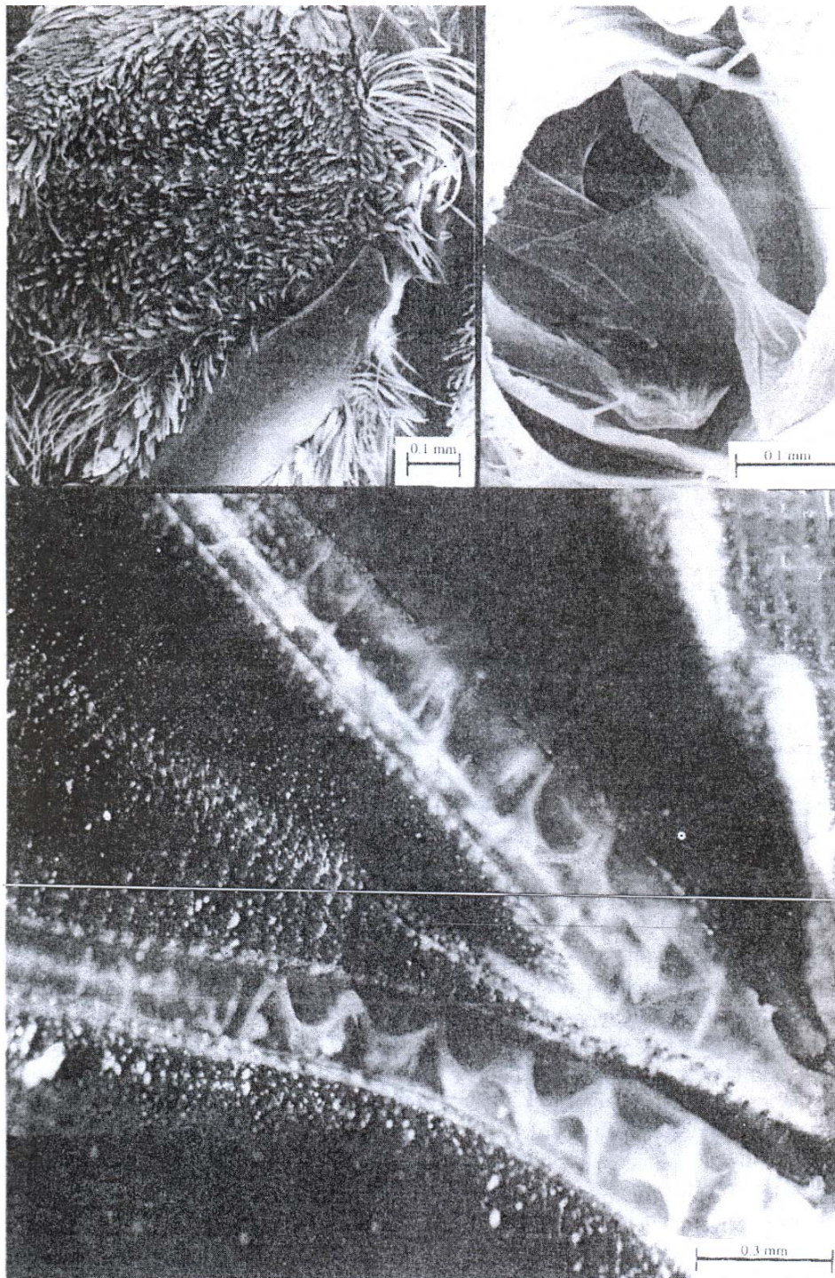
Fig. 18. Details of Hamadryas februa forewings. Bellows: spiral structure inside veins. Above left: intact ear. Above right: inner view of membranous spiral structure.
